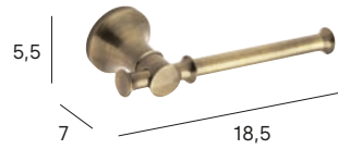
Portarrollos sin tapa Paper holder w/o cover
